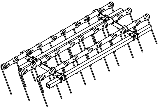
9 FINGER ASSEMBLY SHOWN
