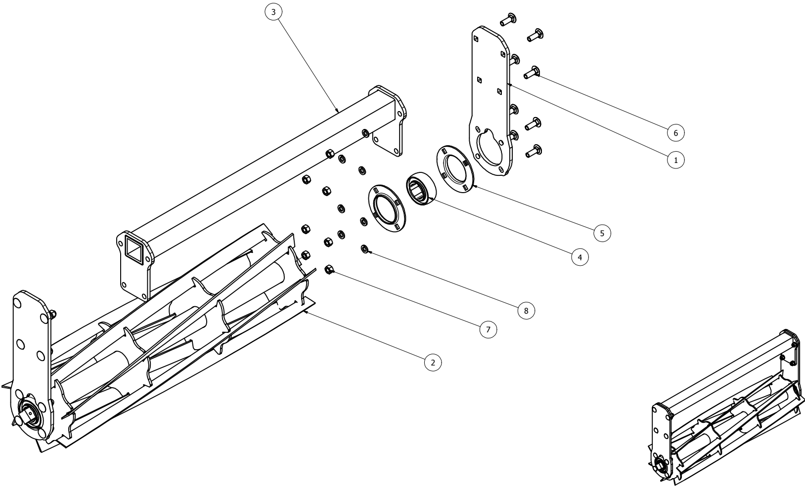
3' BASKET ASSEMBLY SHOWN
