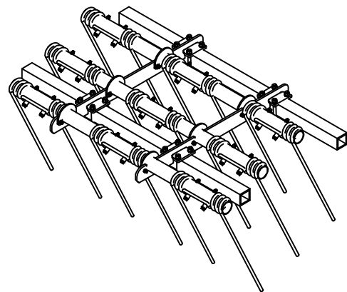
9 FINGER ASSEMBLY SHOWN
