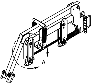
DETAIL A SCALE 0.16 : 1
