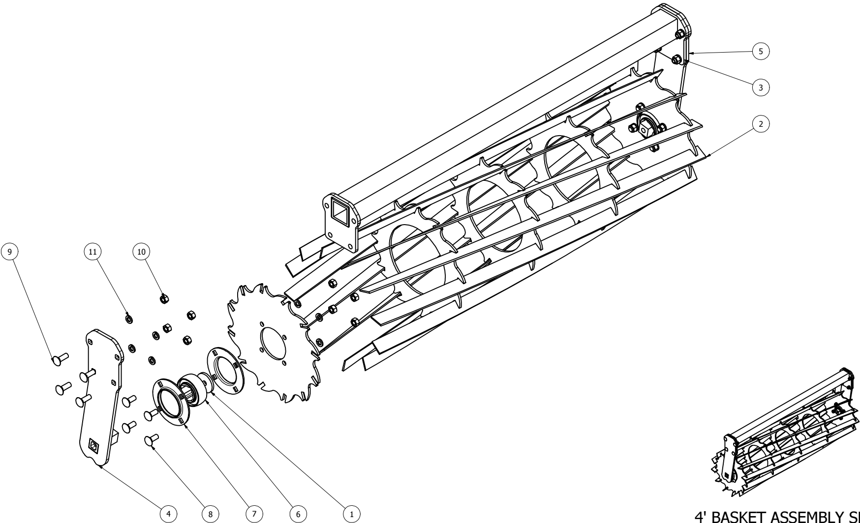
4' BASKET ASSEMBLY SHOWN
