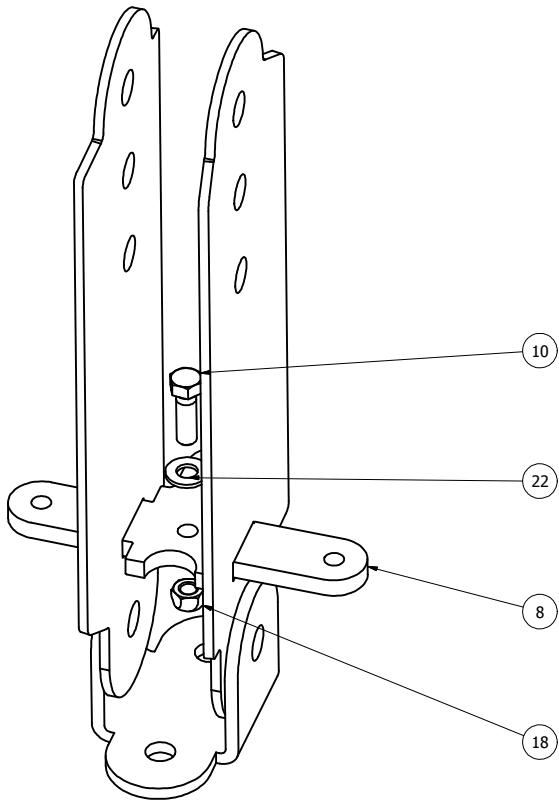
HANGER HARDWARE ASSEMBLY
