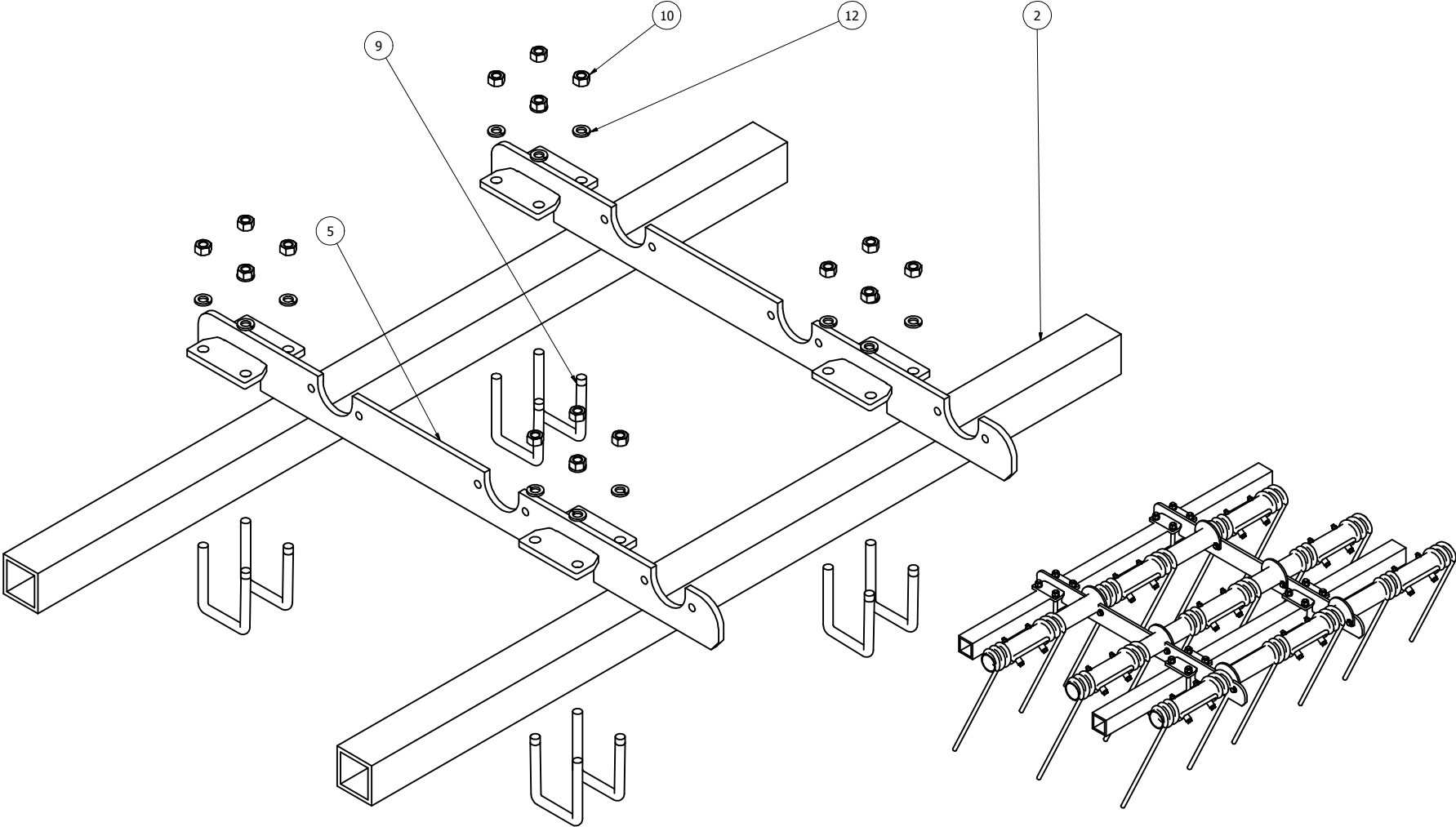
9 FINGER ASSEMBLY SHOWN
