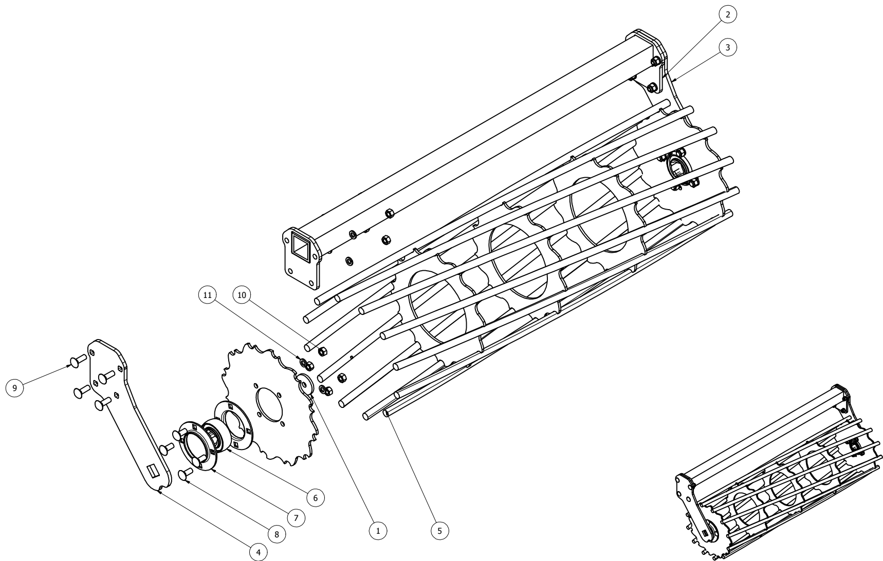
4' BASKET ASSEMBLY SHOWN
