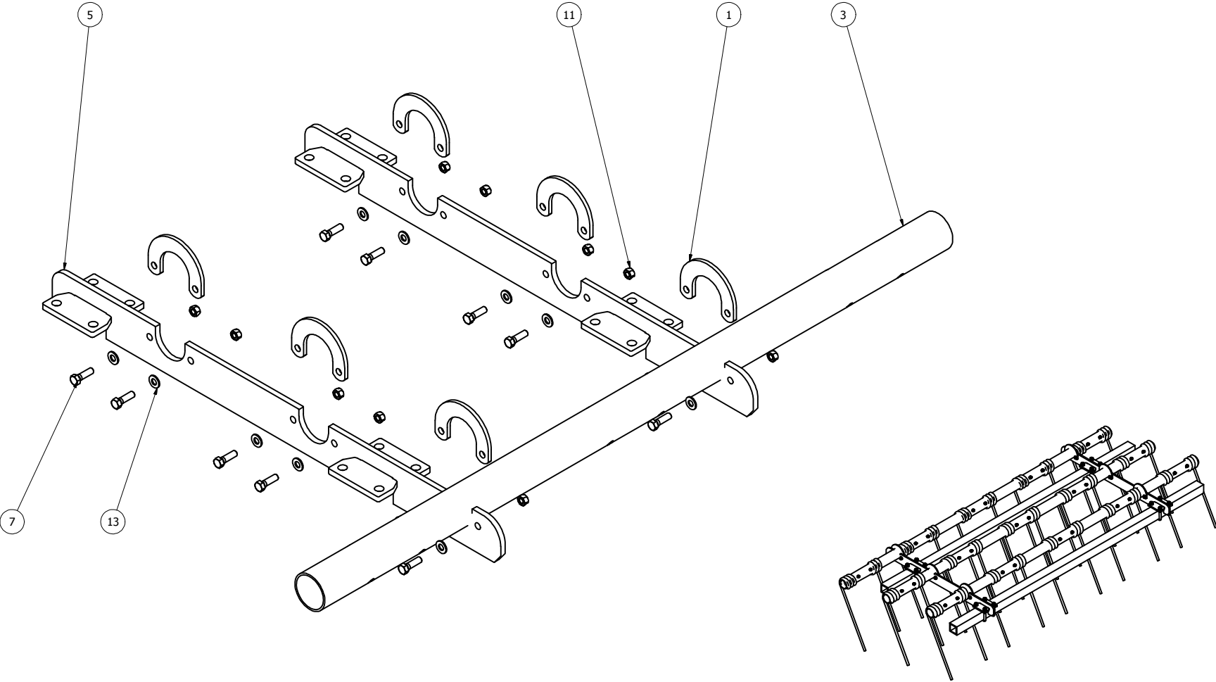
9 FINGER ASSEMBLY SHOWN
